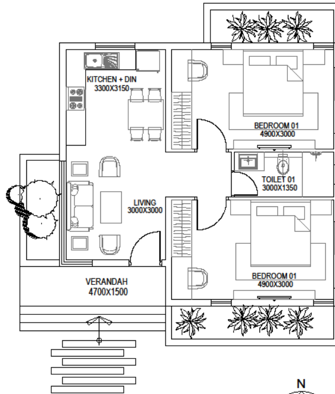
GROUND FLOOR PLAN BUA= 650 SQFT
