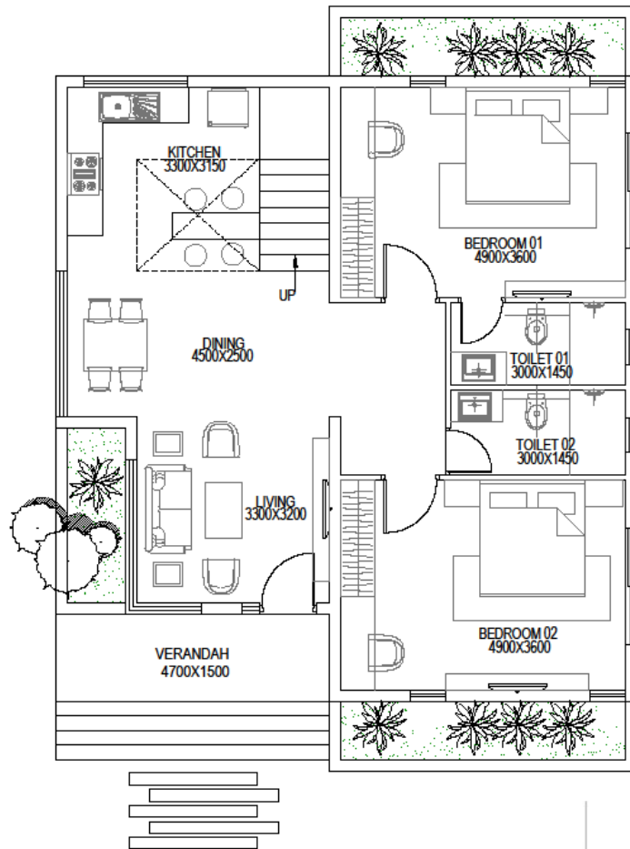
GROUND FLOOR PLAN BUA= 1590 sqft
